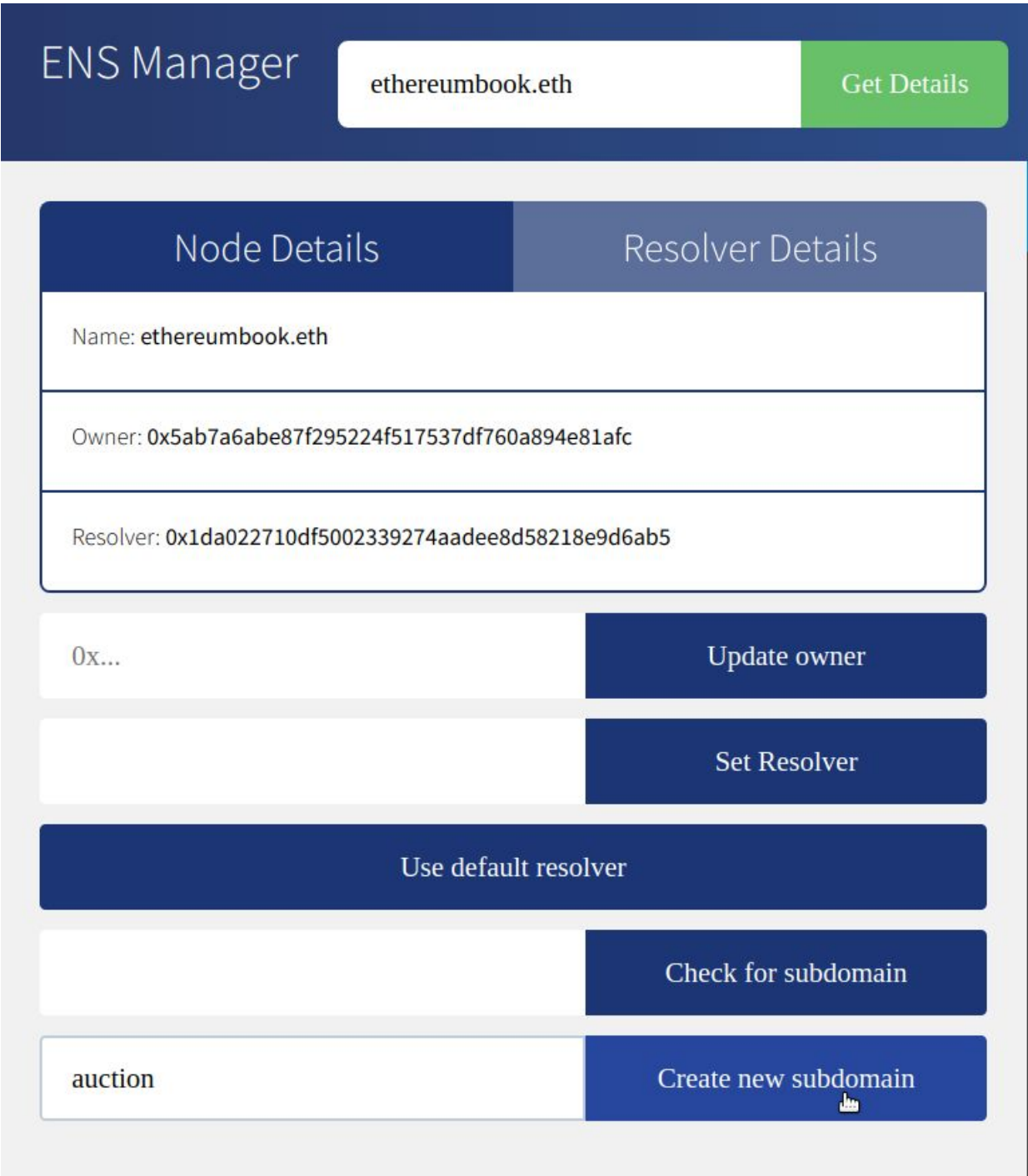
Figure 12-11. Adding the subdomain auction.ethereumbook.eth
