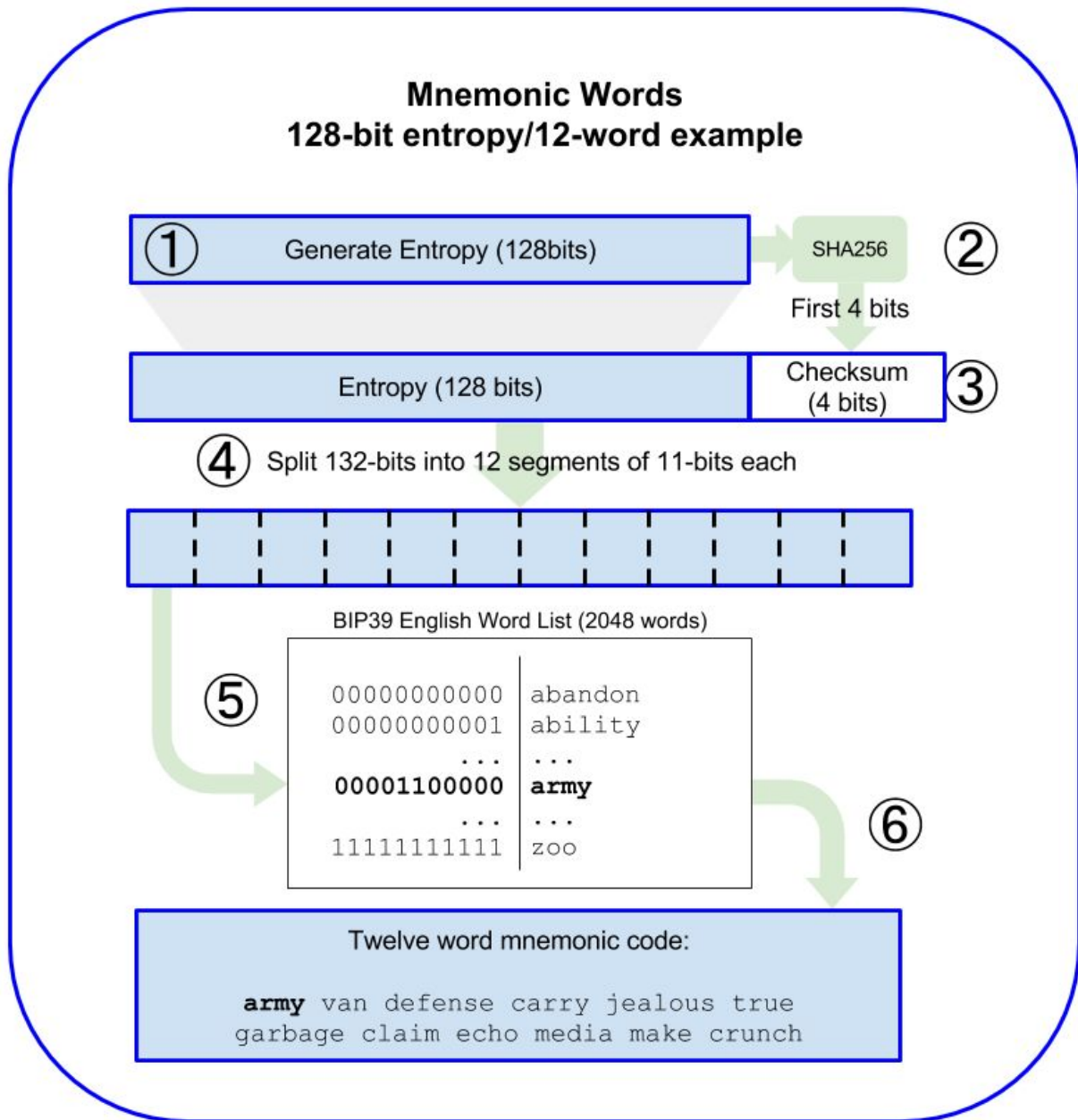
Figure 5-2. Generating entropy and encoding as mnemonic words
