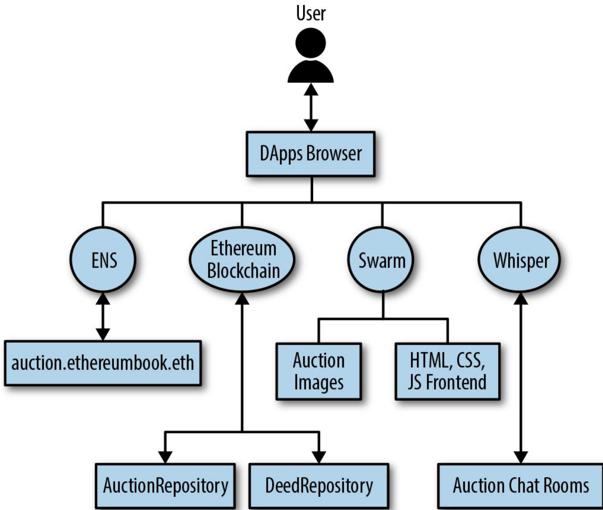
Figure 12-14. Auction DApp architecture
