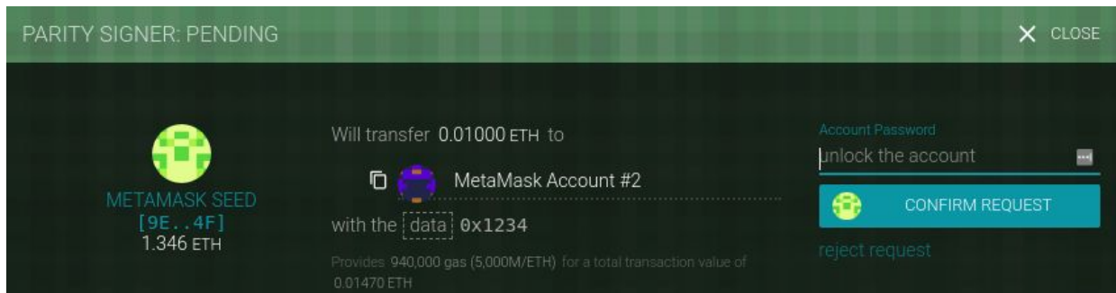
Figure 6-2. Parity wallet showing a transaction with value and data
