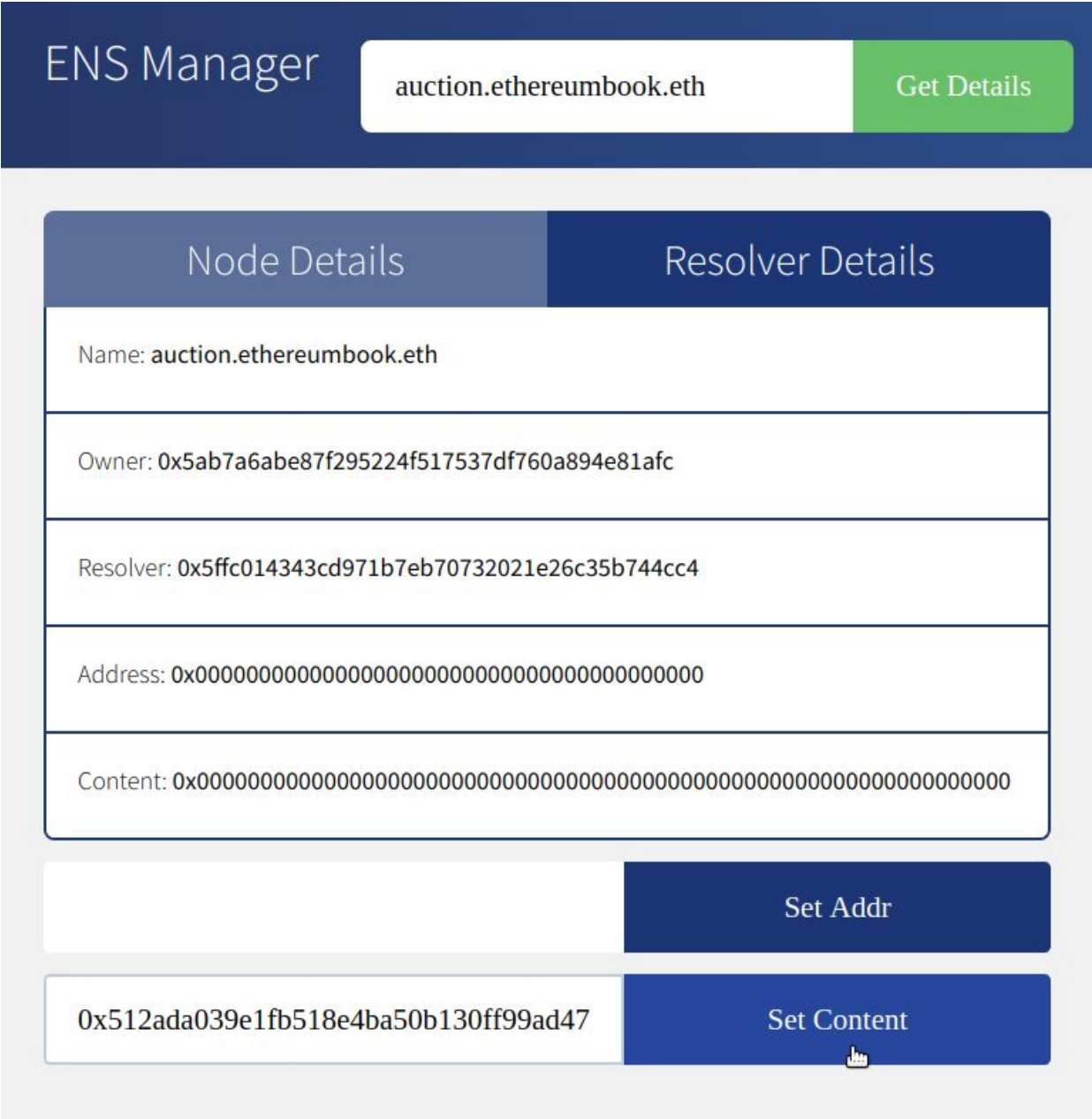
Figure 12-13. Setting the content to return for auction.ethereumbook.eth
