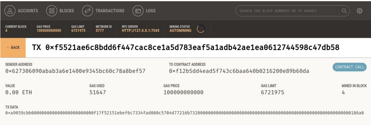
Figure 10-3. METoken transfer on ganache
